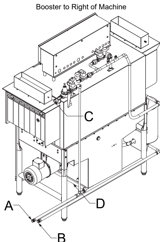
A - Connect to Inlet Water on Booster B - Connect to Outlet Water on Booster
