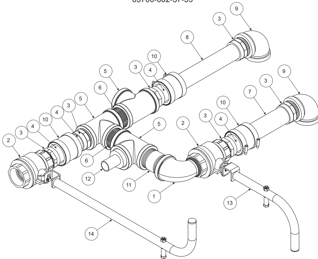
Complete AJ-66 Drain Plumbing Assembly, R-L 05700-002-57-59
