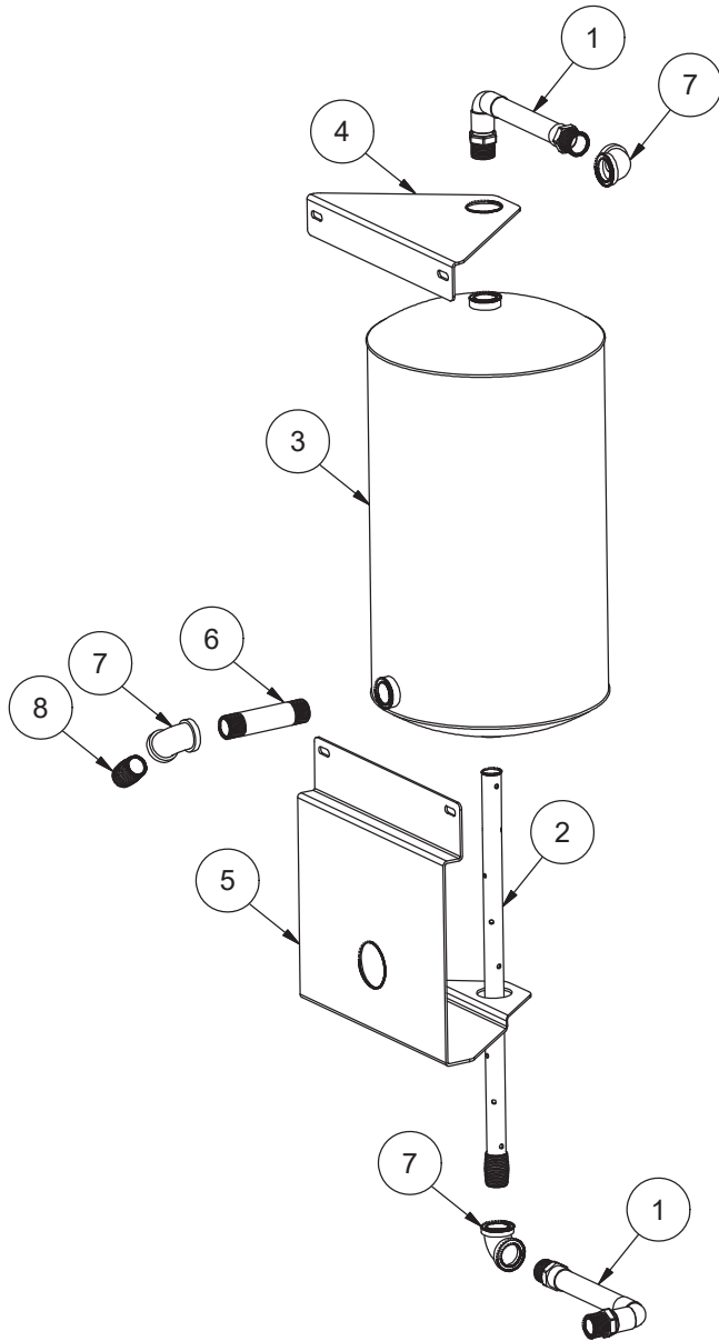
Complete Tank Assembly 05700-002-45-05
