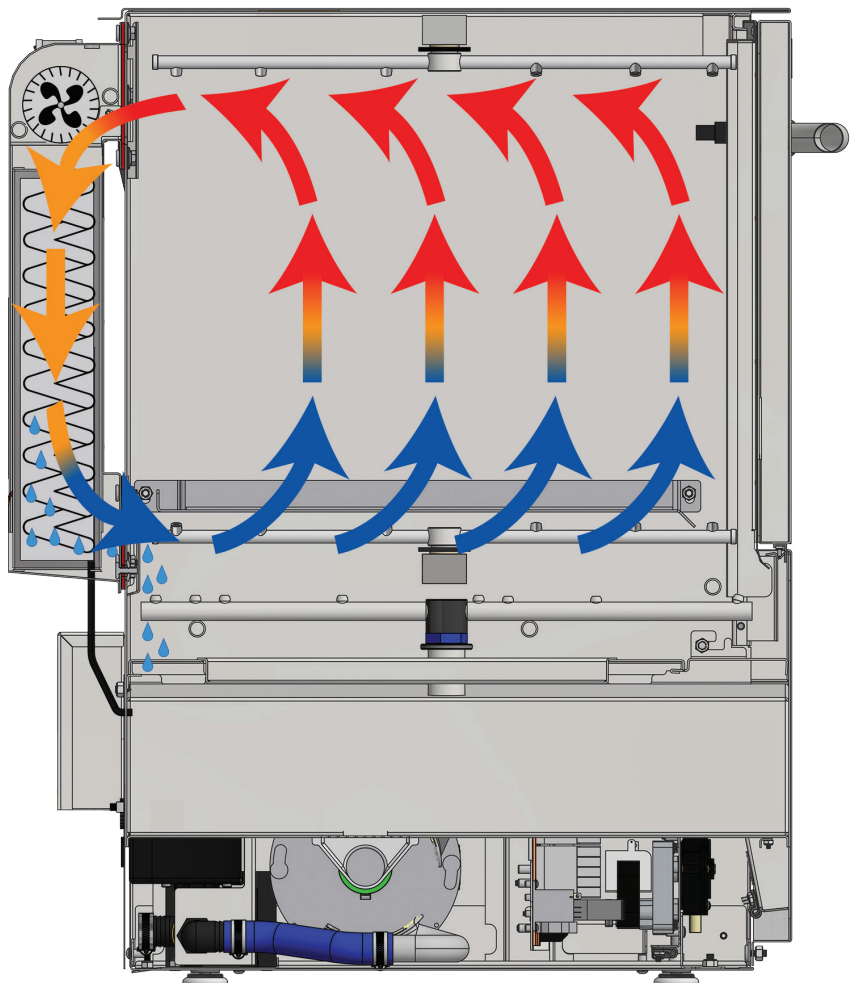
Cutaway side view of the DishStar® HT-E-SEER
