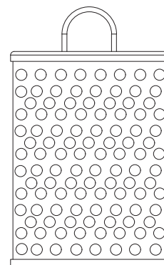
Sump Strainer 05700-002-06-25
