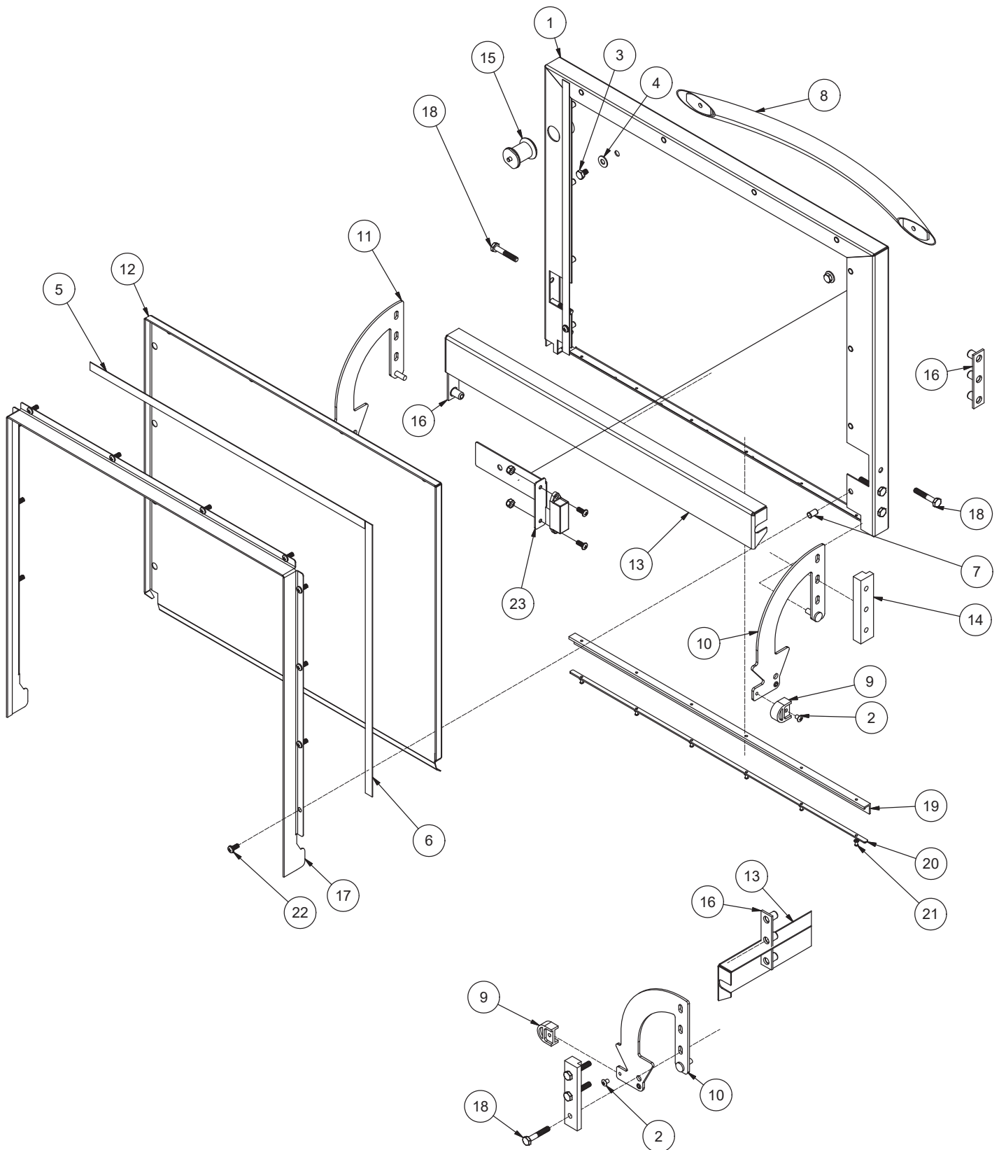
HINGE ASSEMBLY
