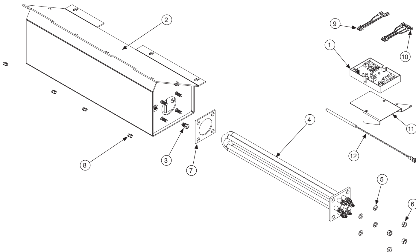
Complete Rinse Tank Assembly 05700-003-31-94
