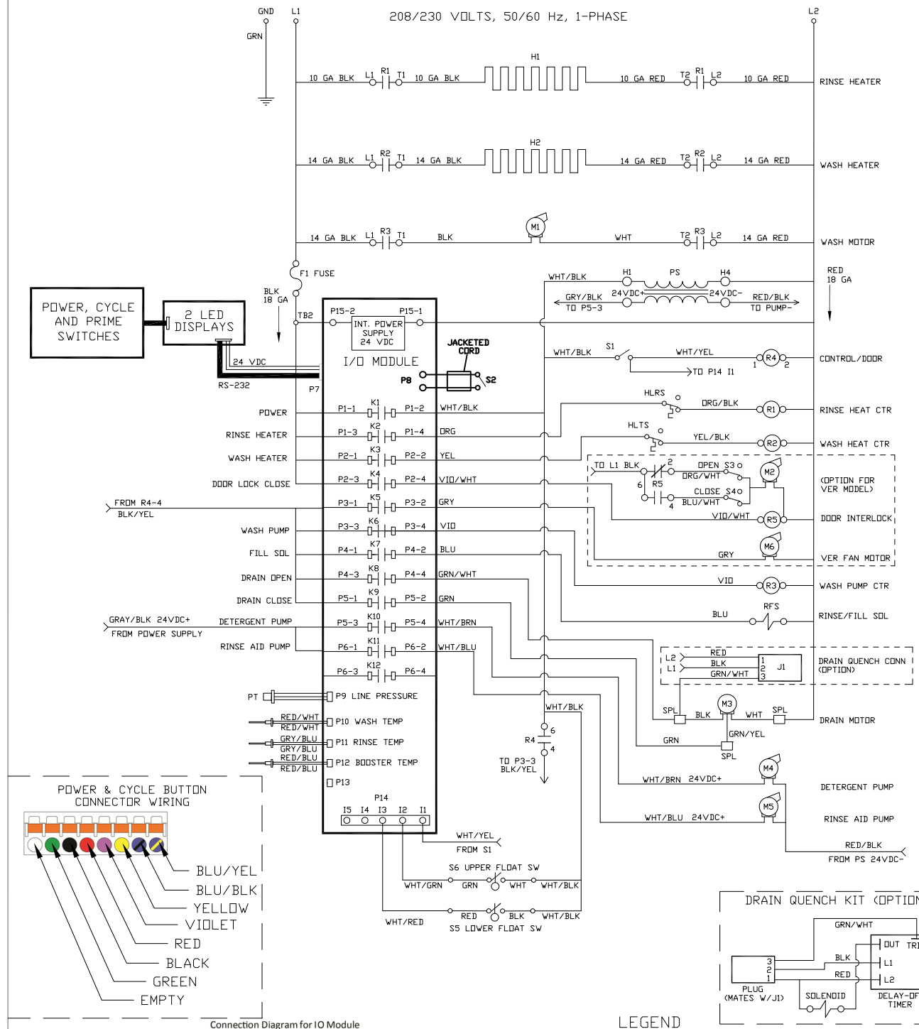
Connection Diagram for IO Module
